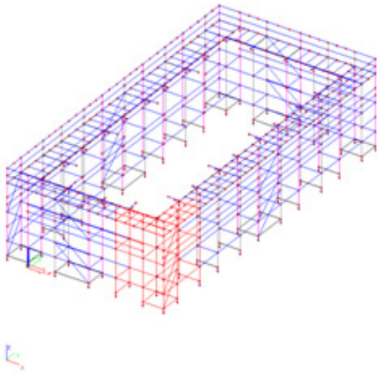
Figure 47: Intelligent 3D scaffolding model
