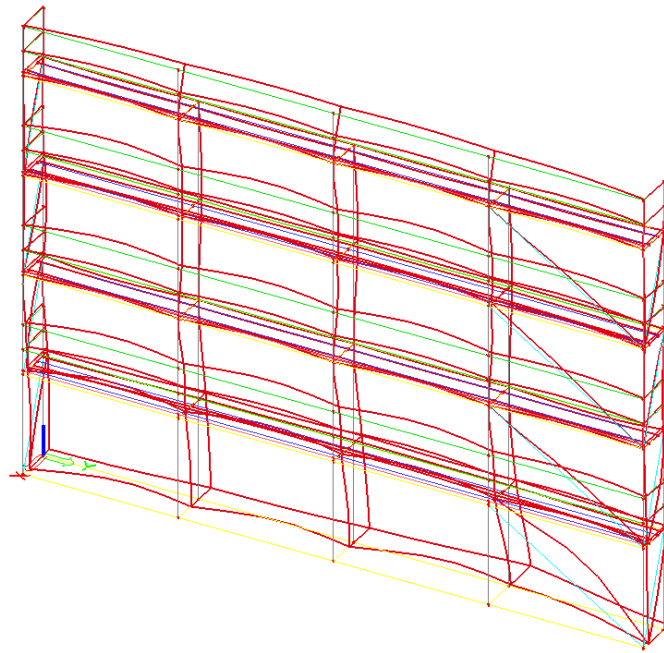
Figure 28: Sliding of base jacks
