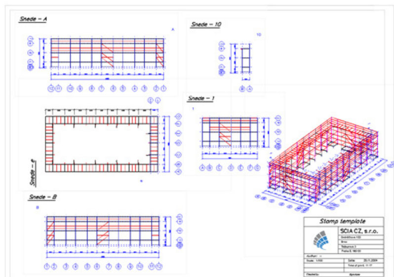
Figure 48: Automatic overview drawings derived from the 3D scaffolding model
