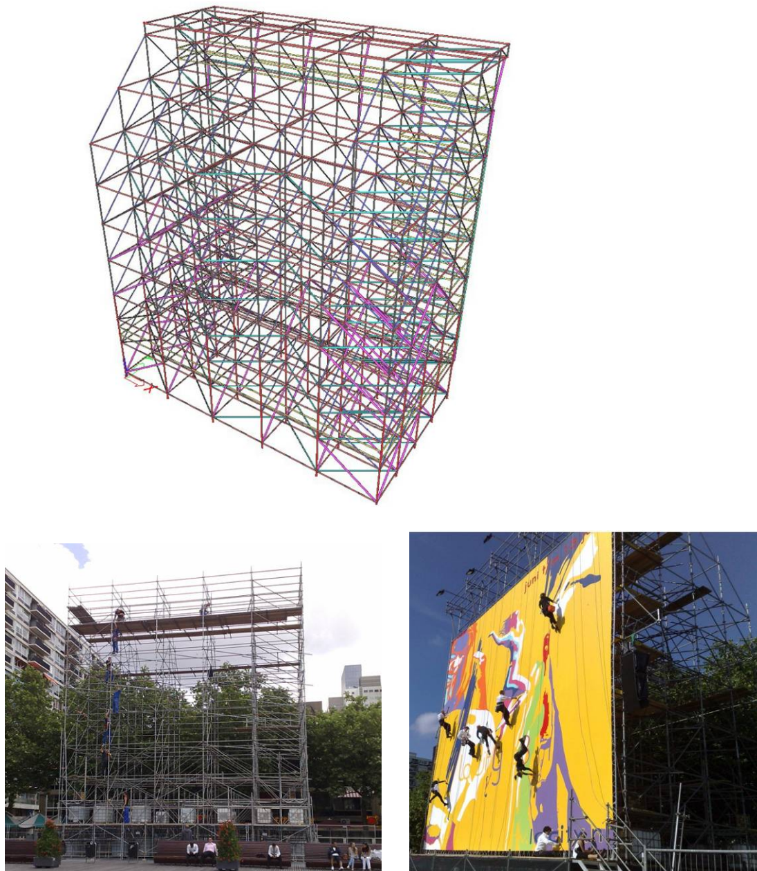
Figure 39: Example of a free standing scaffold modeled and analyzed with SCIA Engineer
