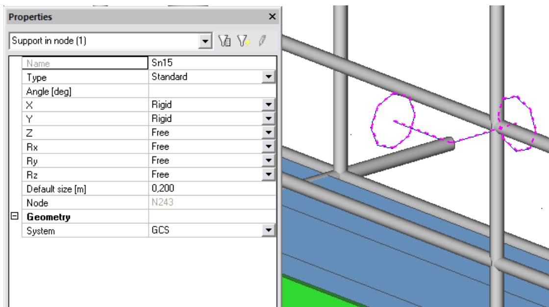
Figure 29: Anchorages in the analysis model
